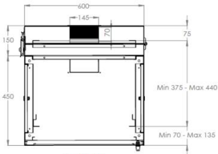
MAX/MIN EQUIPMENT MOUNTING DISTANCE
