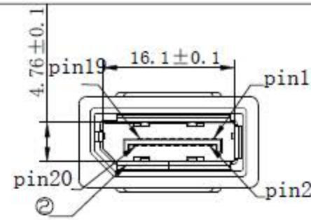
DisplayPort Female
