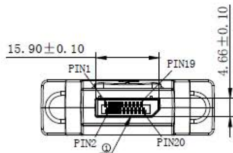
DisplayPort Male
