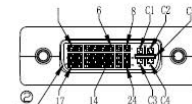
DVI 24+5 Female
