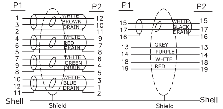
Pin Assignment
