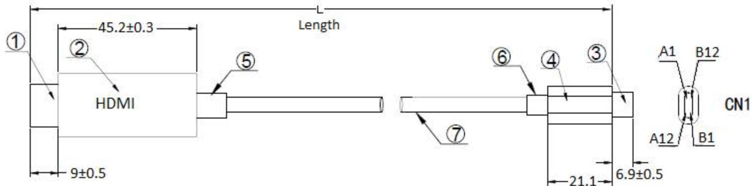
Structure Diagram
